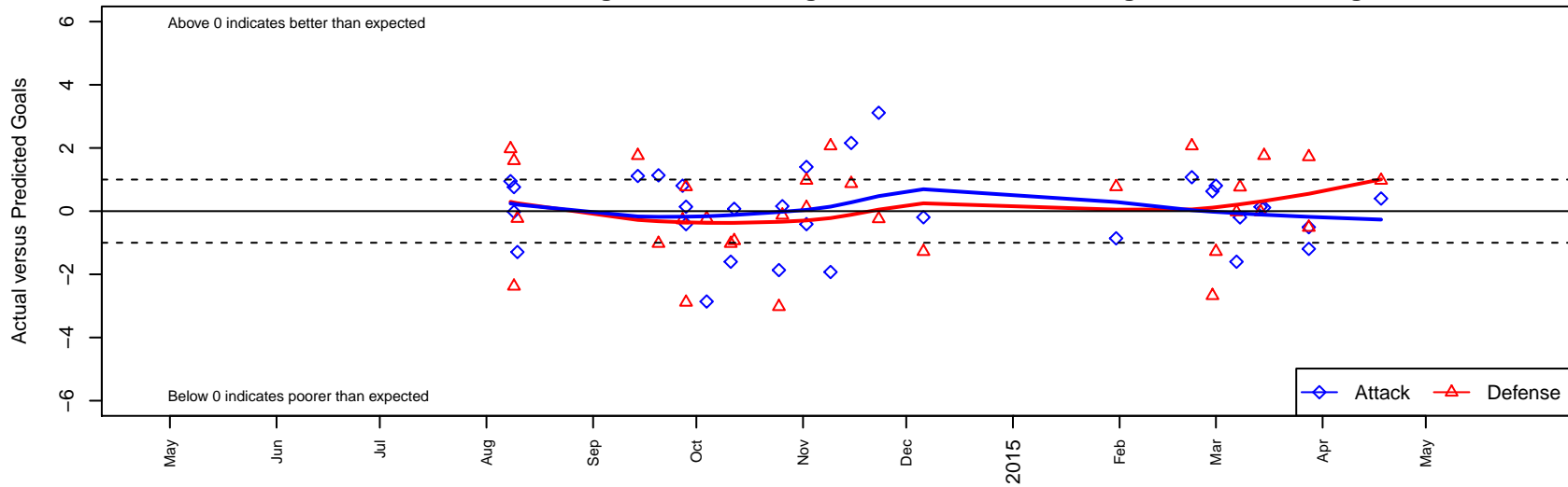
SSC Shadow B B02 Dots are actual minus expected GF (blue circles) and GA (red triangles). Blue line is smoothed change in attack strength. Red is smoothed change in defense strength.
